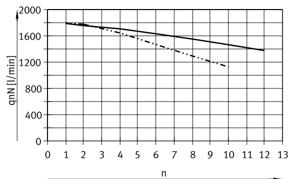
Size 30 – Standard nominal flow rate q_{nN} , with several valves n switched in parallel For 3/2-way valves
