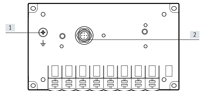
[1] Earthing screw
