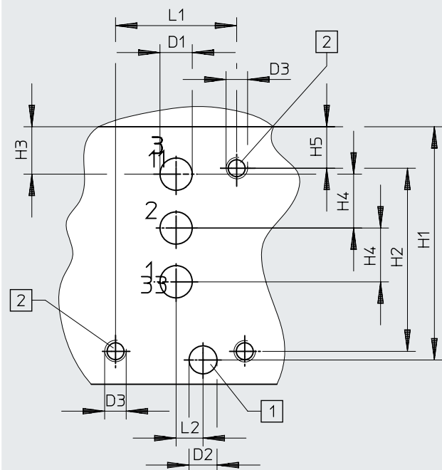
[1] Hole for coding pin, 2.5mm deep [2] Mounting thread, 13 mm deep
