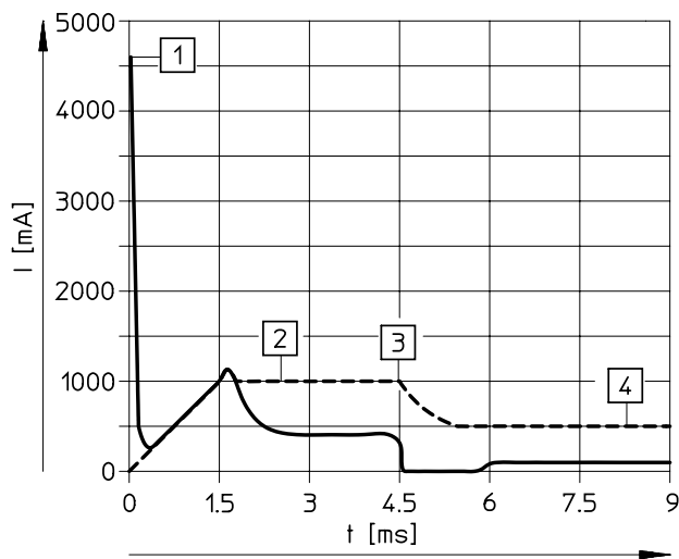
Current curve for valves with fast-switching electronics (MHP2-MS1H)
