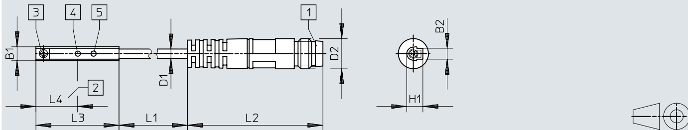
Dimensions – SME-10 plug, connection outlet direction lengthways
