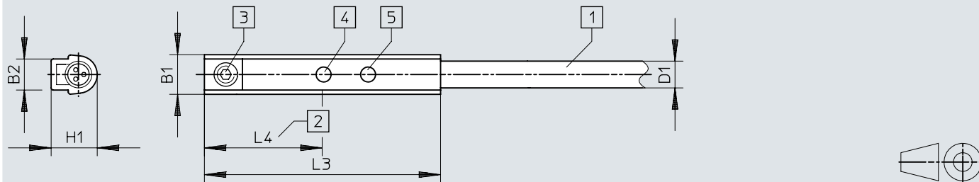
Dimensions – SME-10M-...-L, outlet direction of connection lengthways
