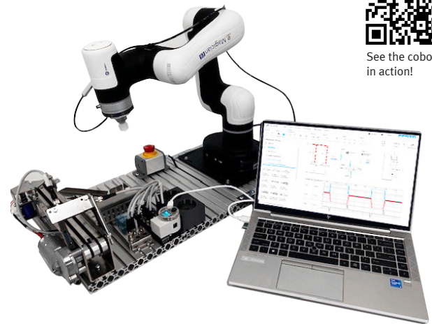
The cobot is displayed alongside the conveyor belt station, seamlessly connected to FluidSIM through the EasyPort device.
