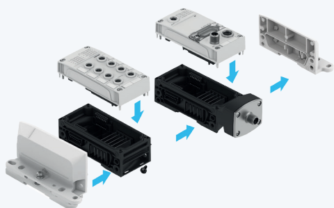
Centralized remote I/O terminals CPX-AP-A
