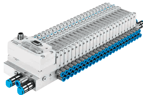
Valve terminal VTUG with plug-in
