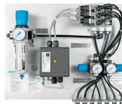
Mounting plate as ready-to-install solution
