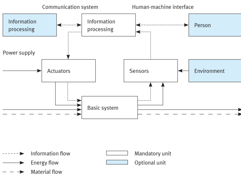
Figure 1: Basic structure of a mechatronic system 1
