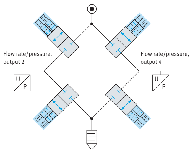
Figure 3: The actuator in the Festo Motion Terminal VTEM is a digital control piston. It can take on the functions of a wide range of mechanical control pistons found in common directional control valves. The control piston consists of a bridge circuit with piezo pilot and diaphragm poppet valves.
